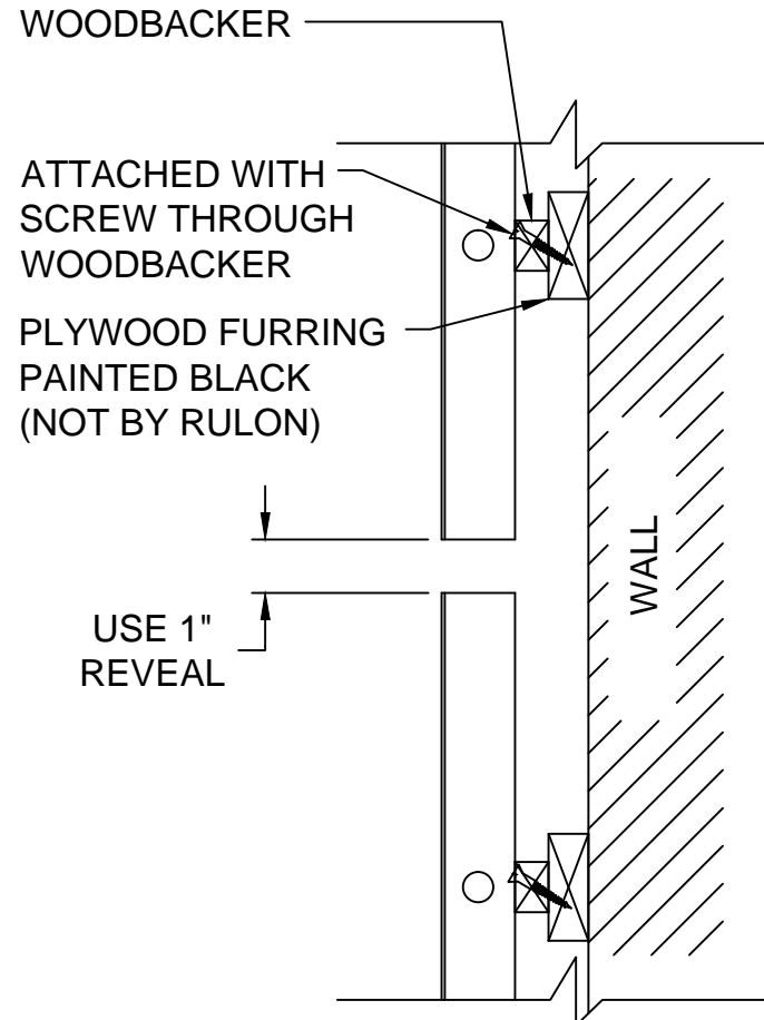
WALL SECTION
